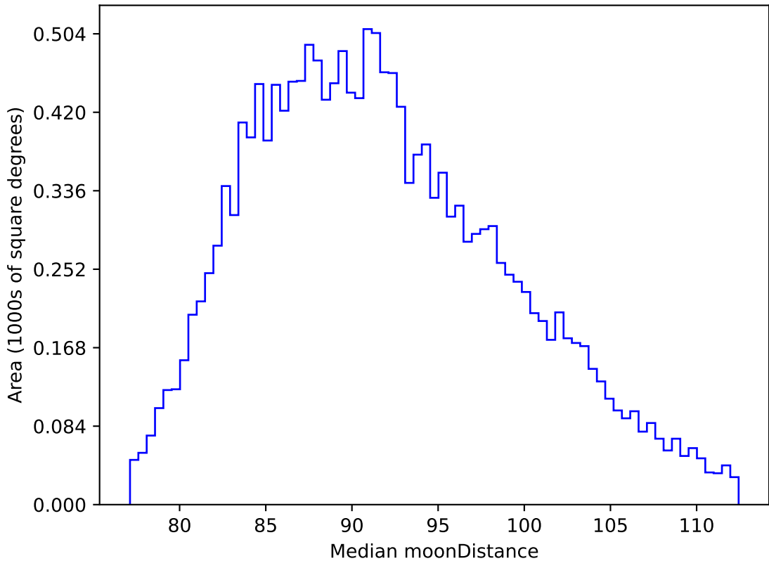
ddf_acor_sf10_lsf40_lsr50_v3.4_10yrs WFD i band: Median moonDistance
