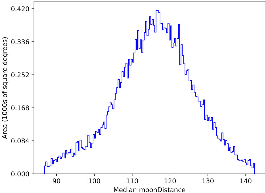
ddf_acor_sf10_lsf40_lsr50_v3.4_10yrs All sky g band: Median moonDistance
