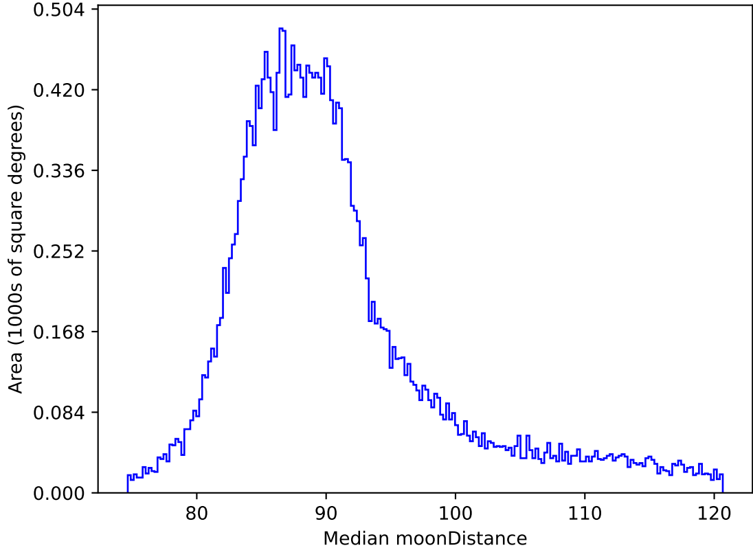
ddf_acor_sf10_lsf40_lsr50_v3.4_10yrs All sky all bands: Median moonDistance
