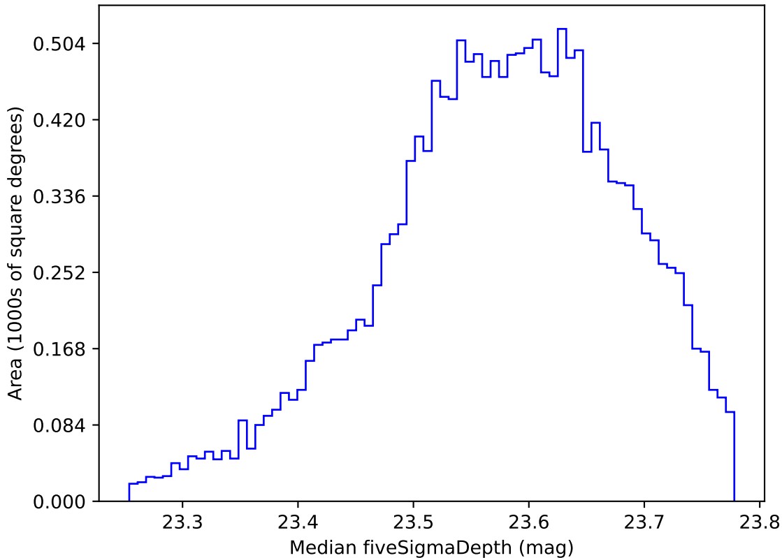
ddf_acor_sf10_lsf40_lsr50_v3.4_10yrs WFD i band: Median fiveSigmaDepth
