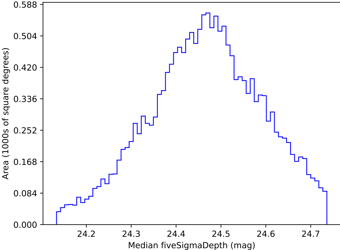
ddf_acor_sf10_lsf40_lsr50_v3.4_10yrs WFD g band: Median fiveSigmaDepth
