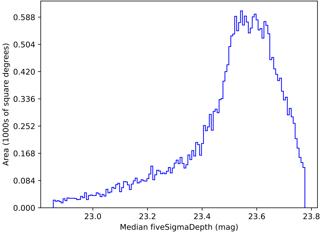
ddf_acor_sf10_lsf40_lsr50_v3.4_10yrs All sky i band: Median fiveSigmaDepth
