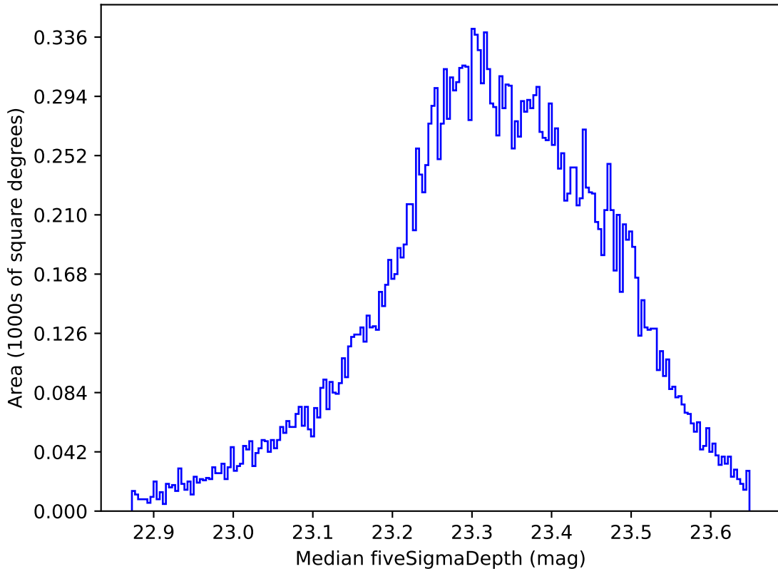
ddf_acor_sf10_lsf40_lsr50_v3.4_10yrs All sky all bands: Median fiveSigmaDepth
