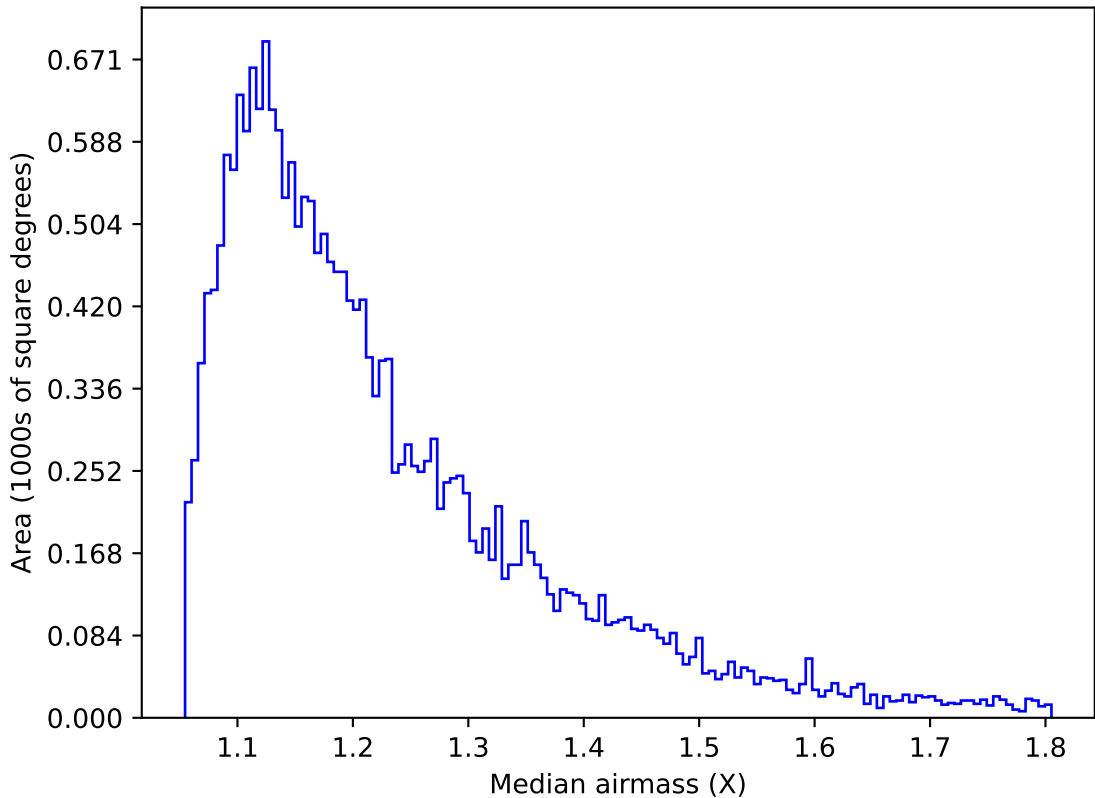
ddf_acor_sf10_lsf40_lsr50_v3.4_10yrs Yr 1 u band: Median airmass
