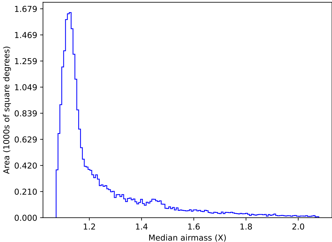
ddf_acor_sf10_lsf40_lsr50_v3.4_10yrs Yr 1 all bands: Median airmass
