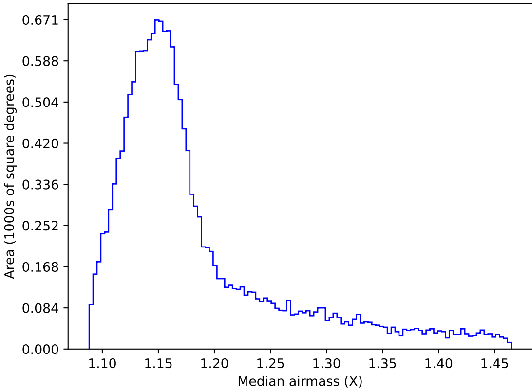
ddf_acor_sf10_lsf40_lsr50_v3.4_10yrs WFD z band: Median airmass
