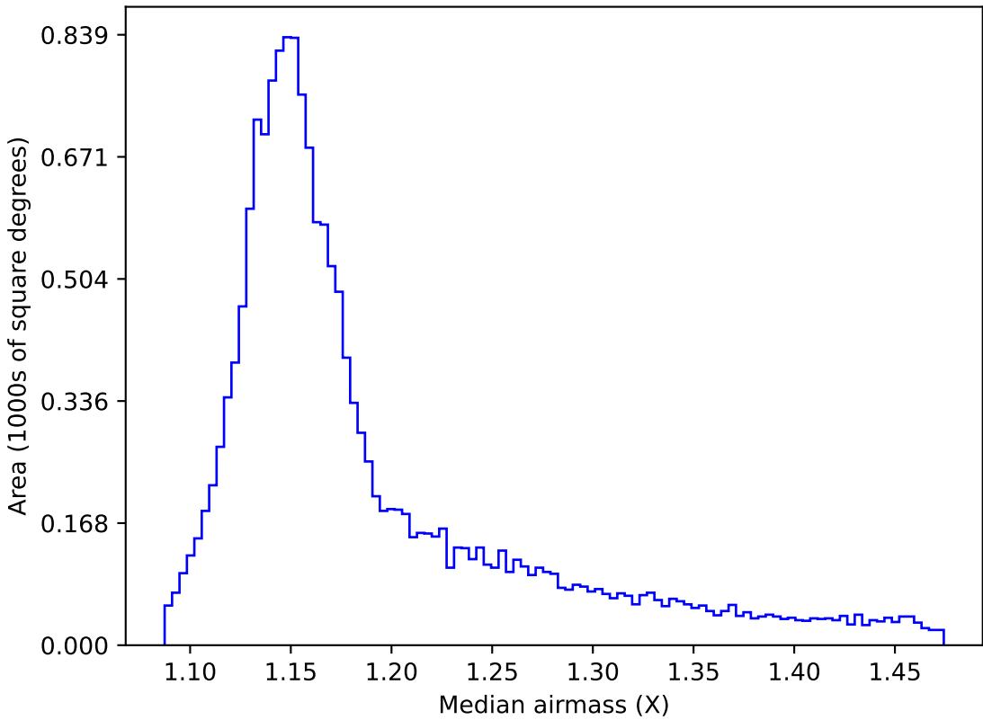
ddf_acor_sf10_lsf40_lsr50_v3.4_10yrs WFD y band: Median airmass
