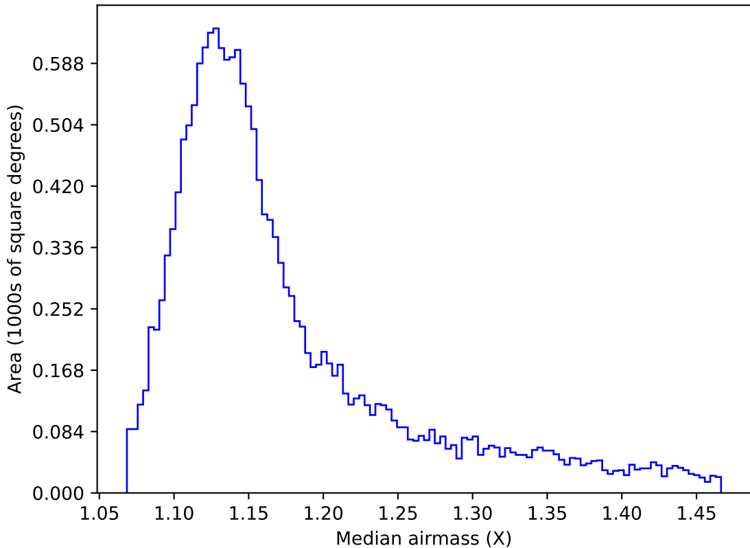
ddf_acor_sf10_lsf40_lsr50_v3.4_10yrs WFD u band: Median airmass
