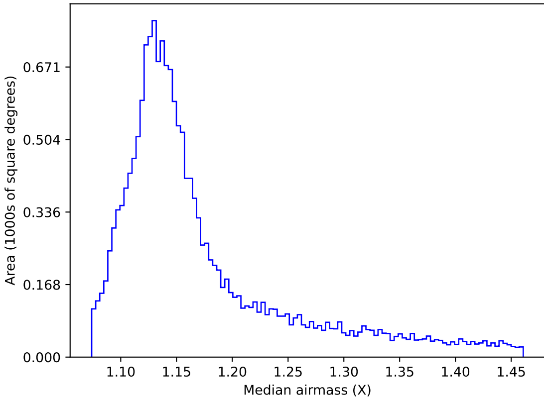
ddf_acor_sf10_lsf40_lsr50_v3.4_10yrs WFD r band: Median airmass
