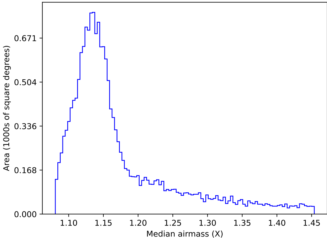
ddf_acor_sf10_lsf40_lsr50_v3.4_10yrs WFD i band: Median airmass
