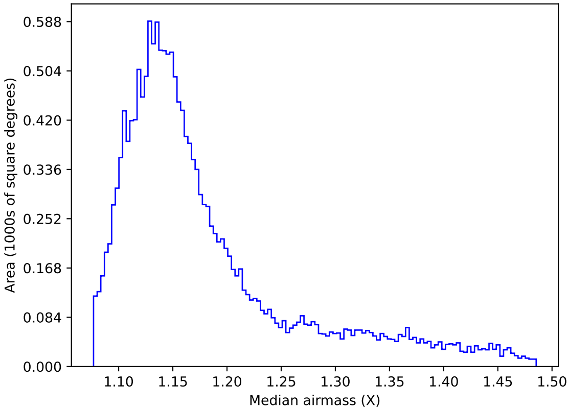
ddf_acor_sf10_lsf40_lsr50_v3.4_10yrs WFD g band: Median airmass
