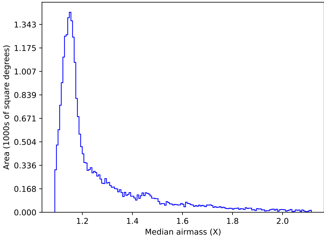
ddf_acor_sf10_lsf40_lsr50_v3.4_10yrs All sky z band: Median airmass
