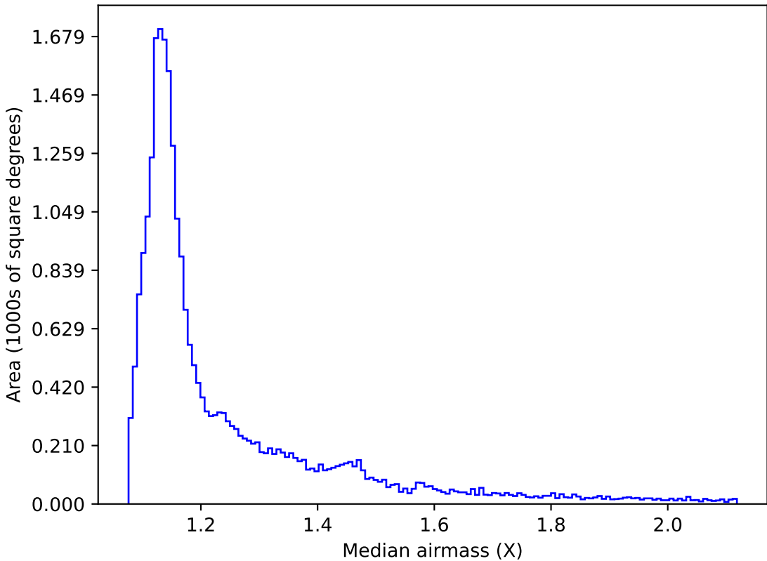
ddf_acor_sf10_lsf40_lsr50_v3.4_10yrs All sky r band: Median airmass
