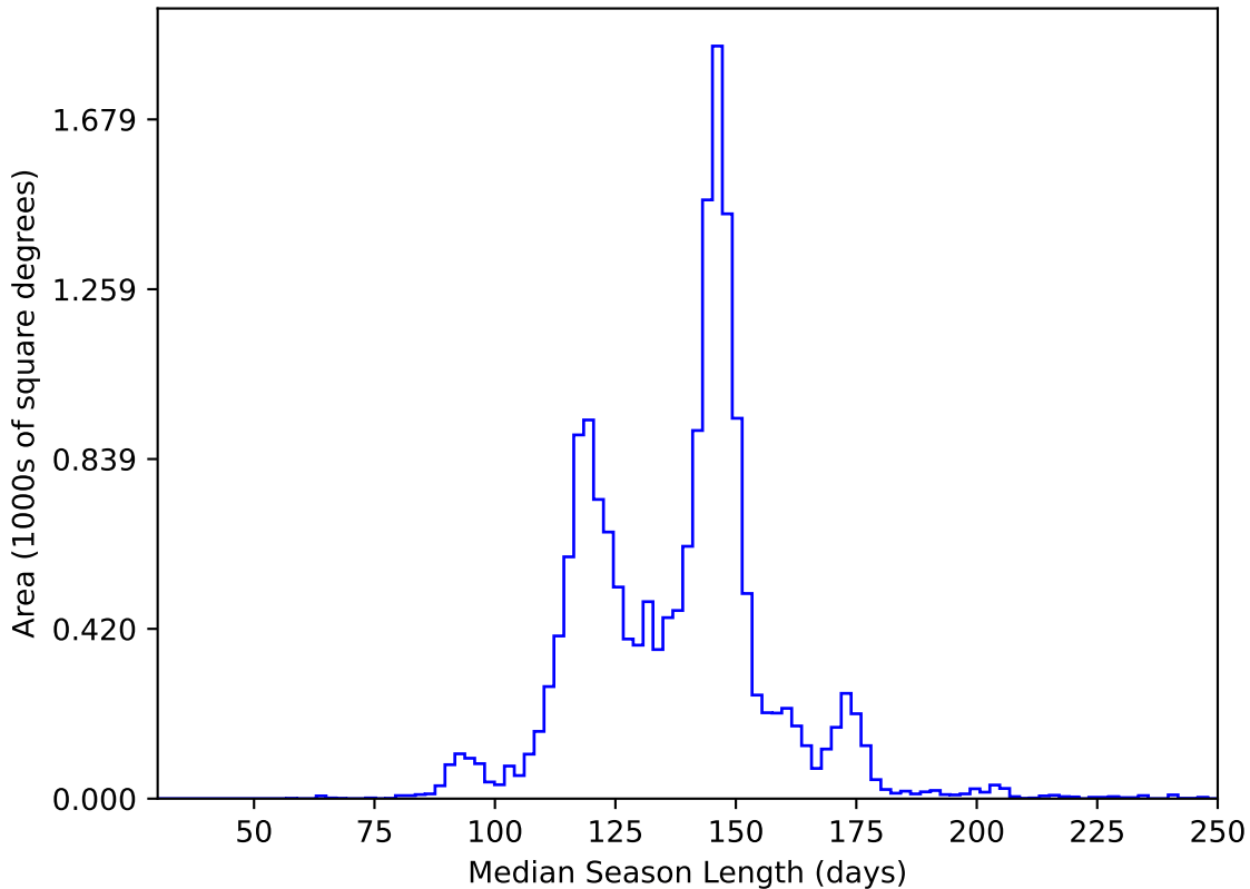
ddf_acor_sf10_lsf40_lsr50_v3.4_10yrs WFD y band: Median Season Length
