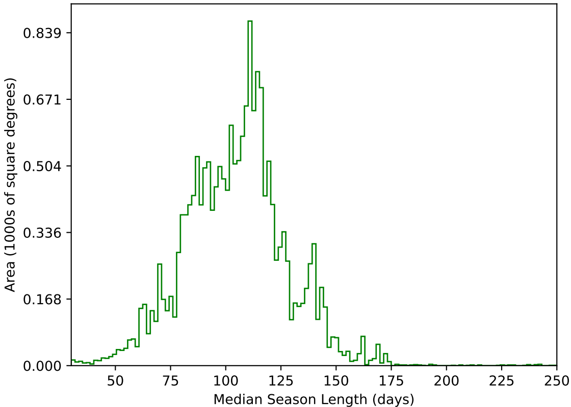
ddf_acor_sf10_lsf40_lsr50_v3.4_10yrs WFD g band: Median Season Length
