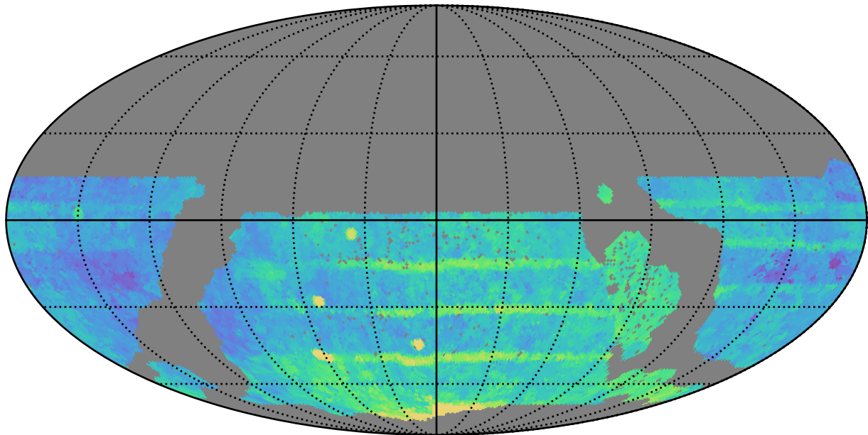
ddf_acor_sf10_lsf40_lsr50_v3.4_10yrs WFD all bands: Median Season Length
