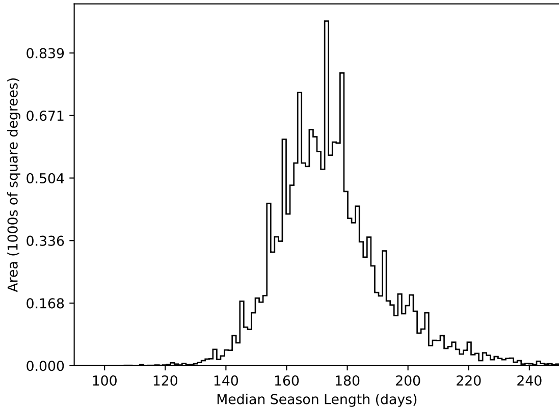
ddf_acor_sf10_lsf40_lsr50_v3.4_10yrs WFD all bands: Median Season Length
