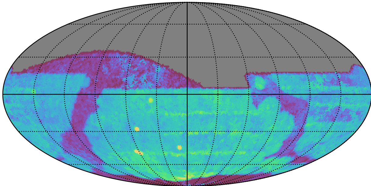
ddf_acor_sf10_lsf40_lsr50_v3.4_10yrs All sky z band: Median Season Length
