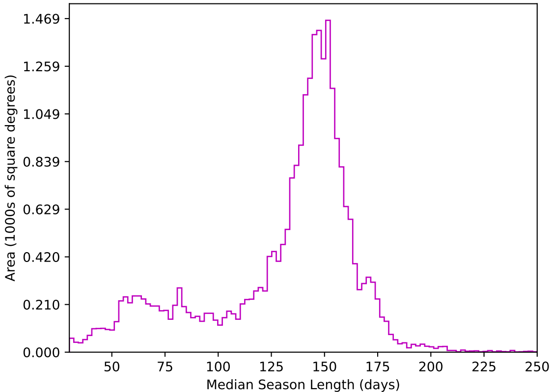
ddf_acor_sf10_lsf40_lsr50_v3.4_10yrs All sky z band: Median Season Length
