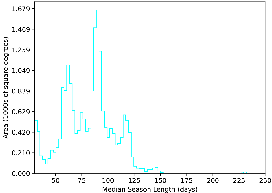
ddf_acor_sf10_lsf40_lsr50_v3.4_10yrs All sky u band: Median Season Length
