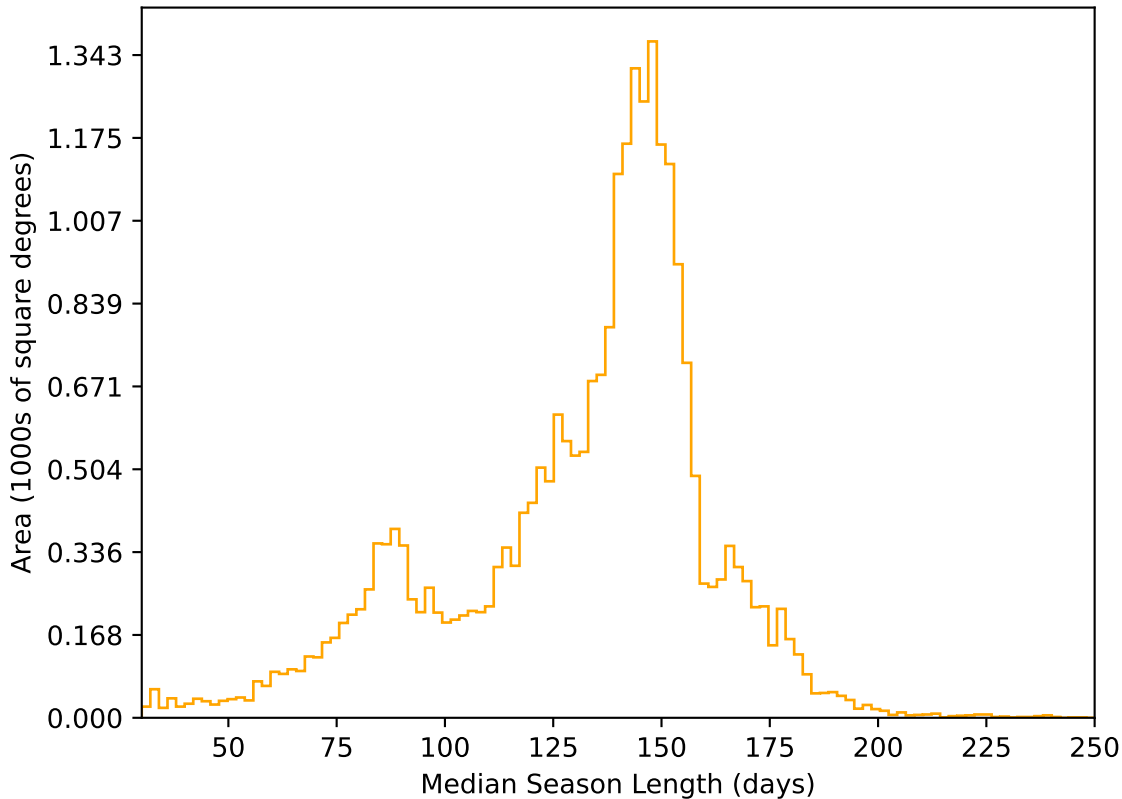
ddf_acor_sf10_lsf40_lsr50_v3.4_10yrs All sky r band: Median Season Length
