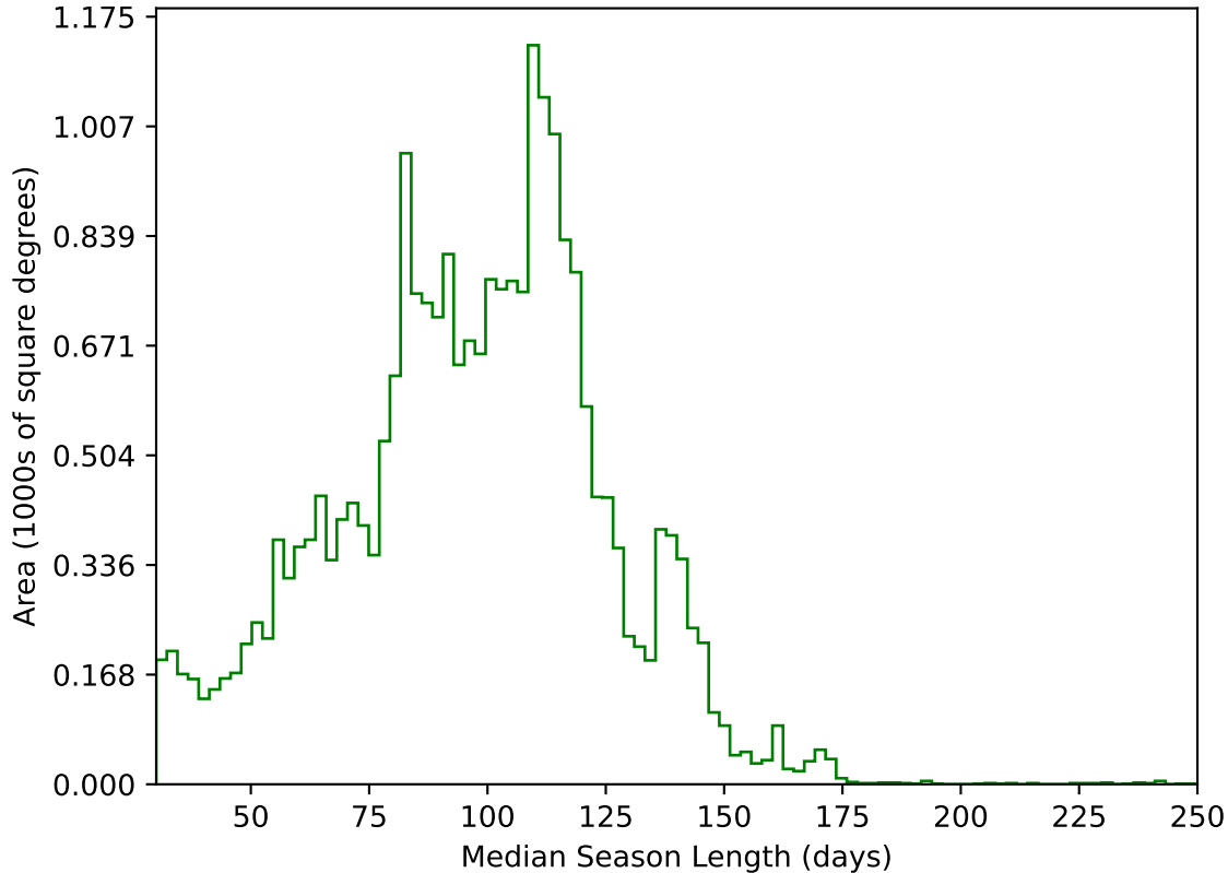
ddf_acor_sf10_lsf40_lsr50_v3.4_10yrs All sky g band: Median Season Length
