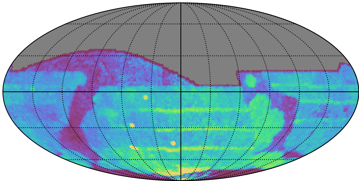
ddf_acor_sf10_lsf40_lsr50_v3.4_10yrs All sky all bands: Median Season Length
