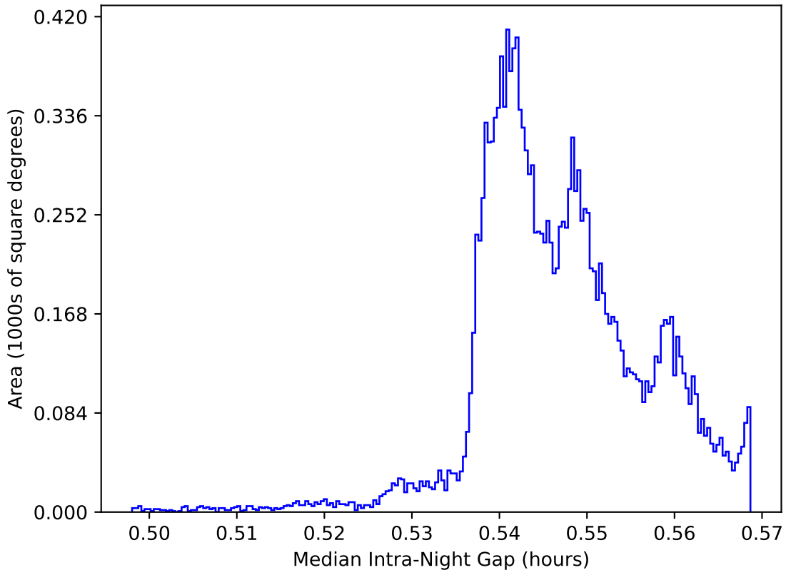
ddf_acor_sf10_ls40_lsr50_v3.4_10yrs WFD: Median Intra-Night Gap
