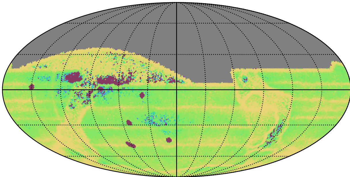
ddf_acor_sf10_lsf40_lsr50_v3.4_10yrs All sky: Median Intra-Night Gap
