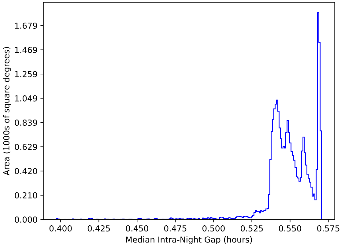
ddf_acor_sf10_lsf40_lsr50_v3.4_10yrs All sky: Median Intra-Night Gap
