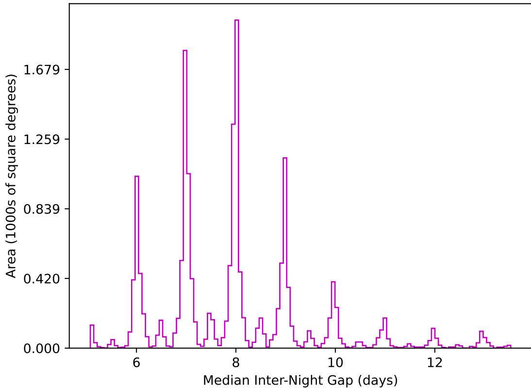
ddf_acor_sf10_lsf40_lsr50_v3.4_10yrs WFD z band: Median Inter-Night Gap
