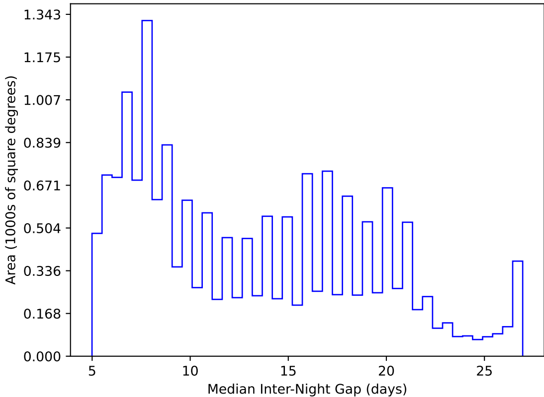
ddf_acor_sf10_lsf40_lsr50_v3.4_10yrs WFD y band: Median Inter-Night Gap
