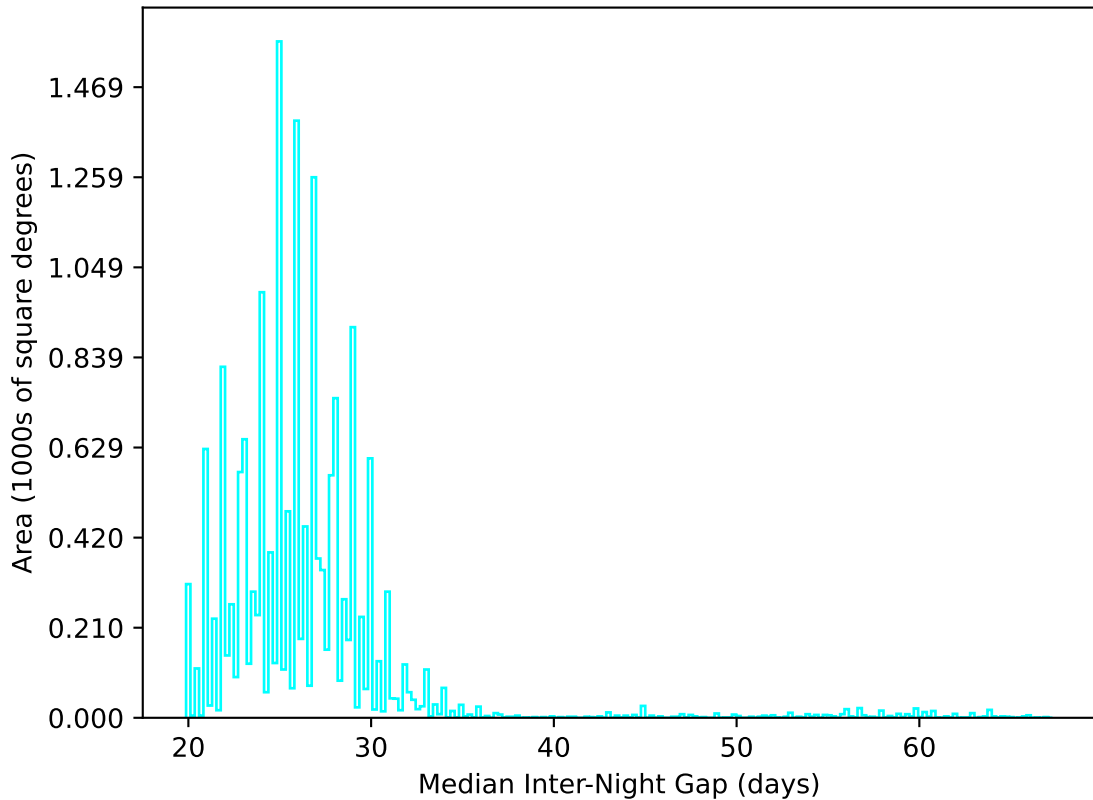
ddf_acor_sf10_lsf40_lsr50_v3.4_10yrs WFD u band: Median Inter-Night Gap
