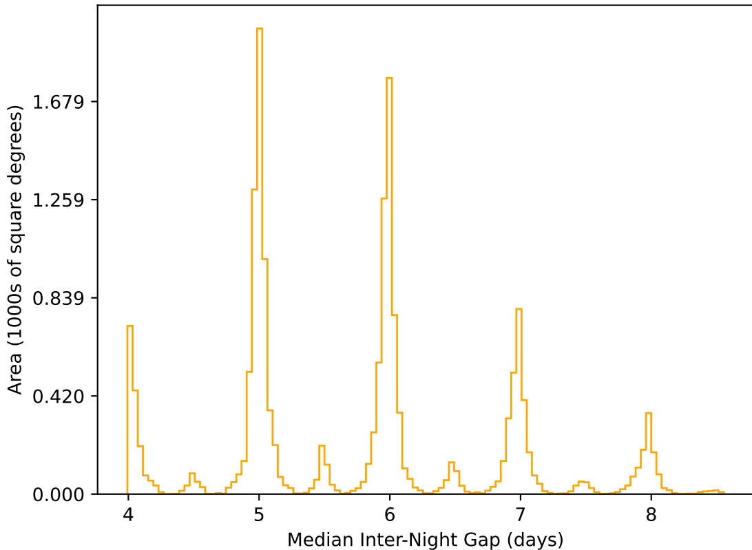
ddf_acor_sf10_lsf40_lsr50_v3.4_10yrs WFD r band: Median Inter-Night Gap
