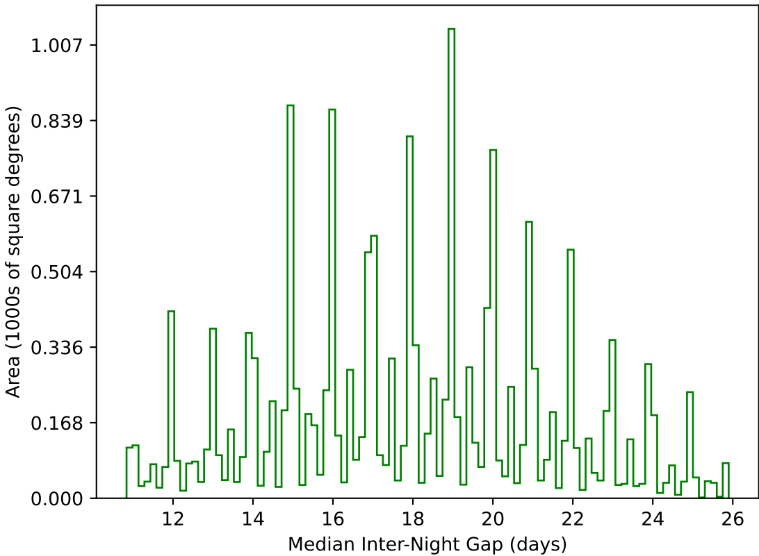
ddf_acor_sf10_lsf40_lsr50_v3.4_10yrs WFD g band: Median Inter-Night Gap
