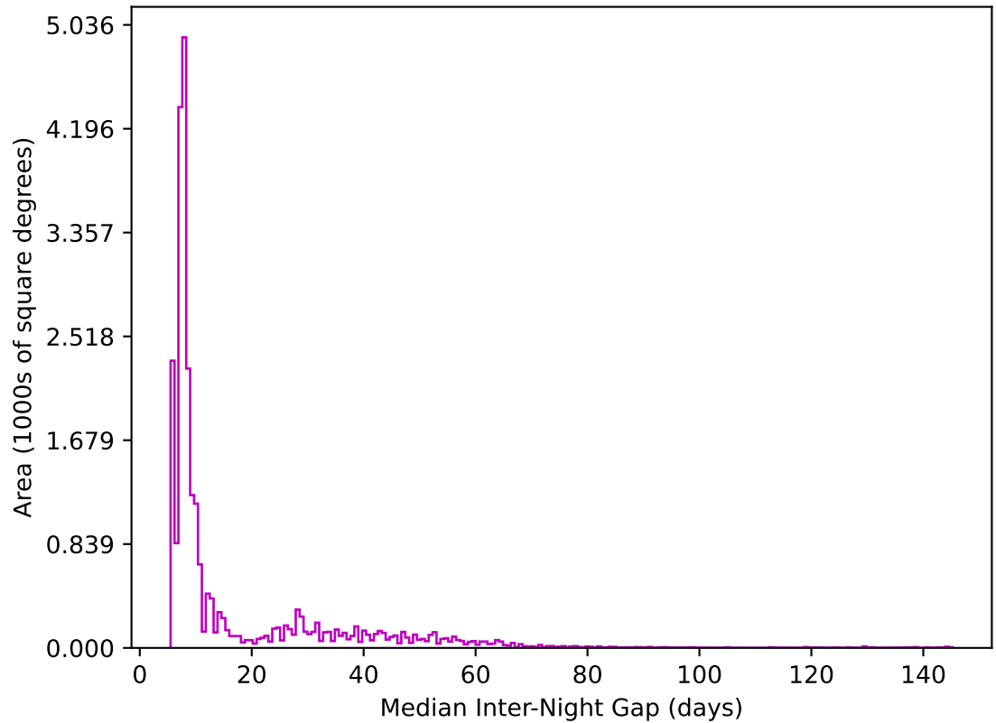
ddf_acor_sf10_lsf40_lsr50_v3.4_10yrs All sky z band: Median Inter-Night Gap
