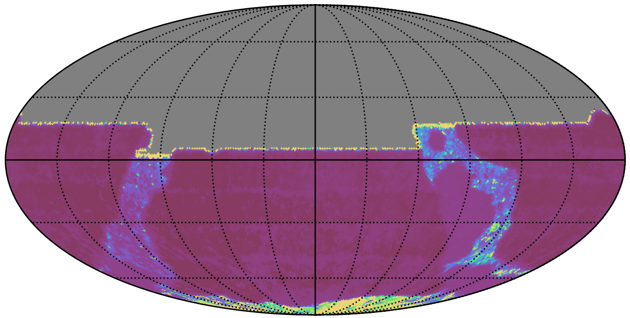
ddf_acor_sf10_lsf40_lsr50_v3.4_10yrs All sky y band: Median Inter-Night Gap
