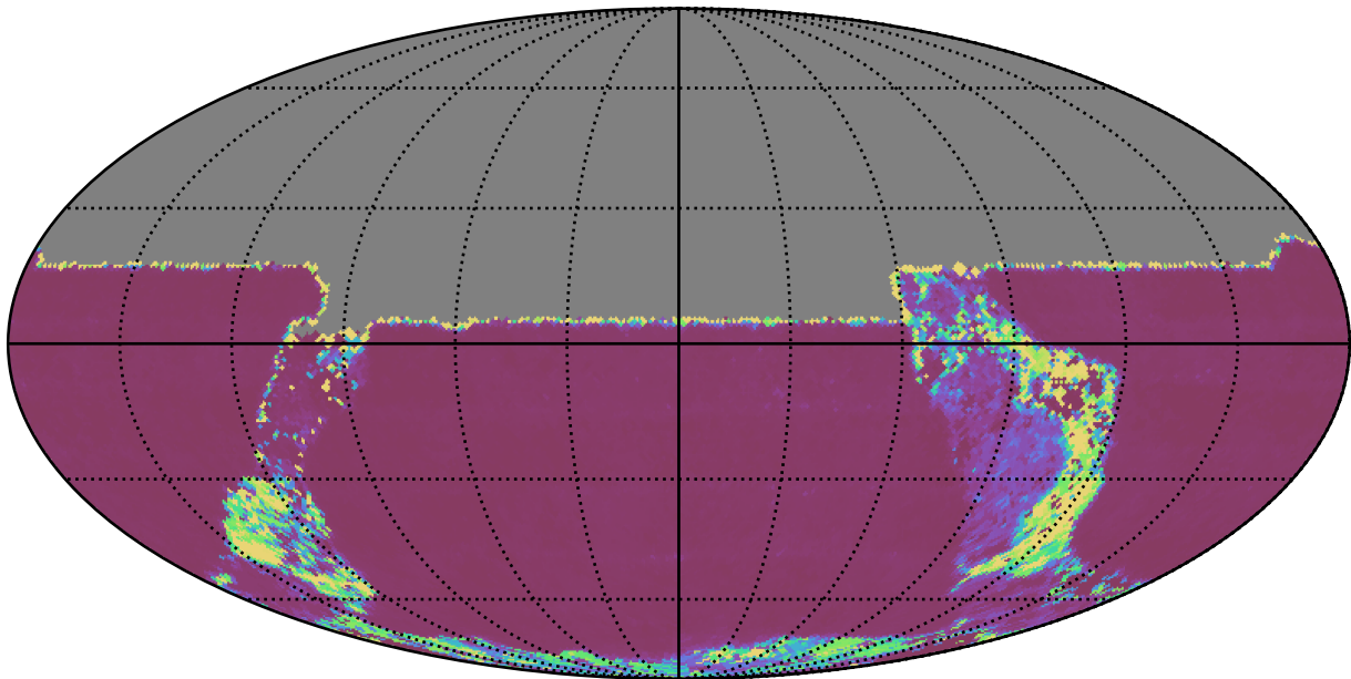
ddf_acor_sf10_lsf40_lsr50_v3.4_10yrs All sky u band: Median Inter-Night Gap
