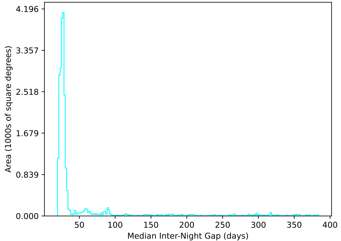
ddf_acor_sf10_lsf40_lsr50_v3.4_10yrs All sky u band: Median Inter-Night Gap
