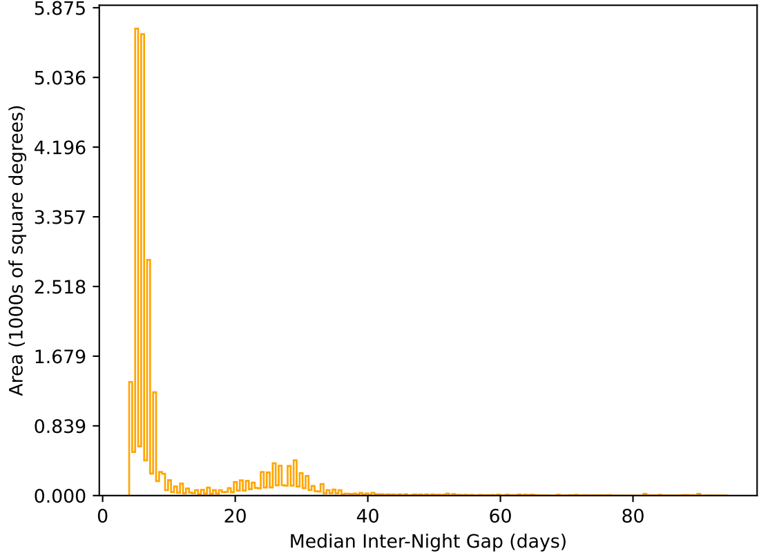
ddf_acor_sf10_lsf40_lsr50_v3.4_10yrs All sky r band: Median Inter-Night Gap
