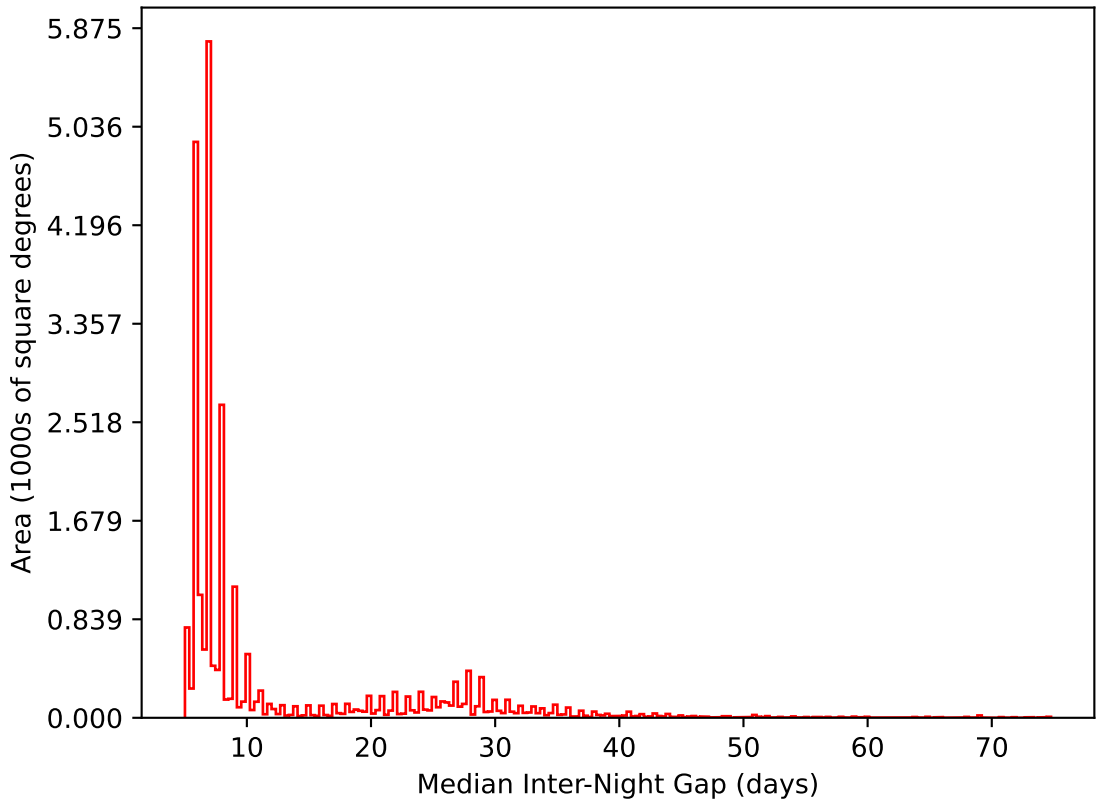
ddf_acor_sf10_lsf40_lsr50_v3.4_10yrs All sky i band: Median Inter-Night Gap
