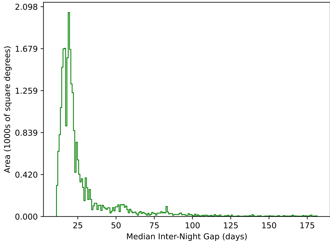
ddf_acor_sf10_lsf40_lsr50_v3.4_10yrs All sky g band: Median Inter-Night Gap
