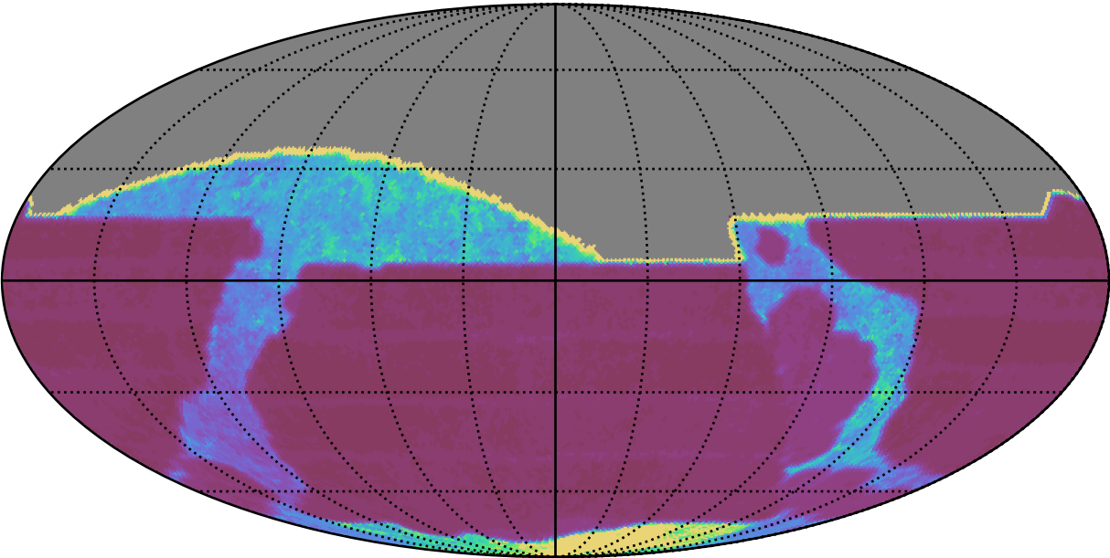
ddf_acor_sf10_lsf40_lsr50_v3.4_10yrs All sky all bands: Median Inter-Night Gap
