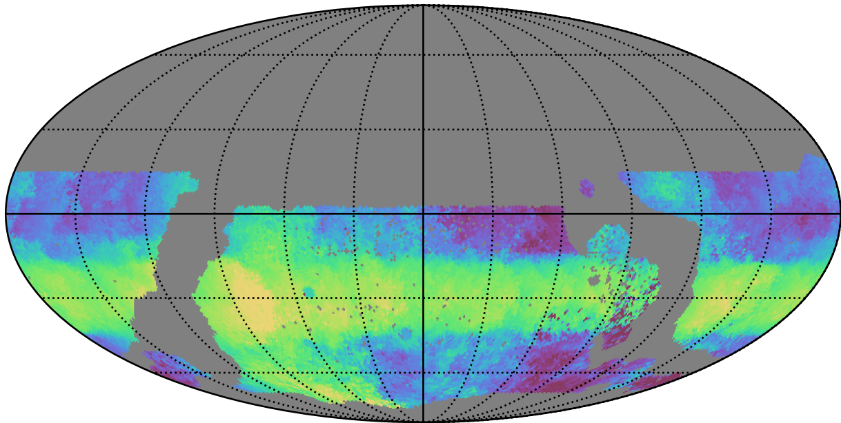
ddf_acor_sf10_lsf40_lsr50_v3.4_10yrs WFD u band: Median HA
