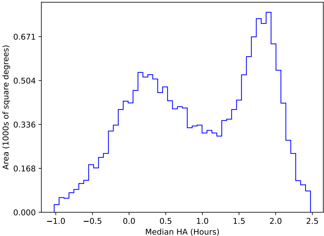
ddf_acor_sf10_lsf40_lsr50_v3.4_10yrs WFD u band: Median HA
