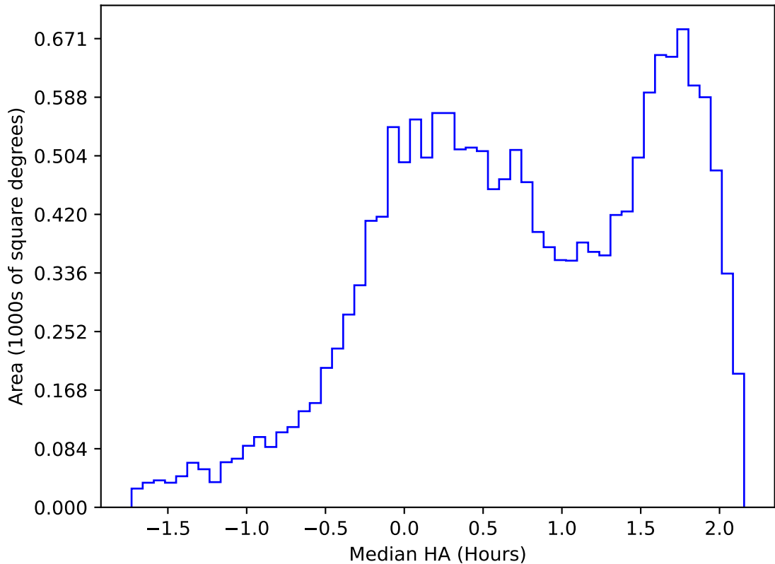
ddf_acor_sf10_lsf40_lsr50_v3.4_10yrs WFD g band: Median HA
