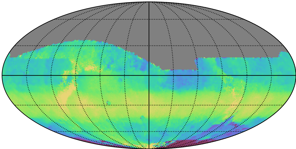
ddf_acor_sf10_lsf40_lsr50_v3.4_10yrs All sky z band: Median HA
