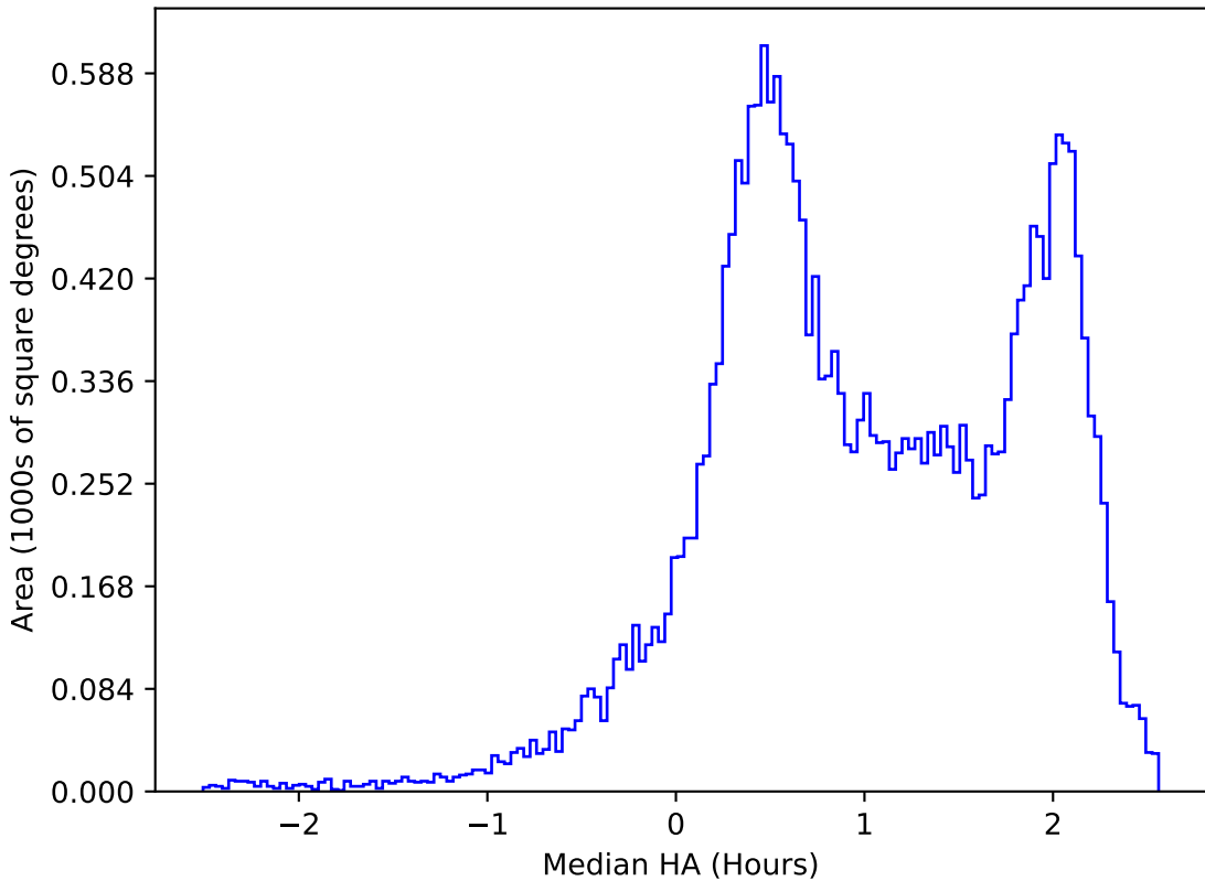
ddf_acor_sf10_ls40_lsr50_v3.4_10yrs All sky z band: Median HA
