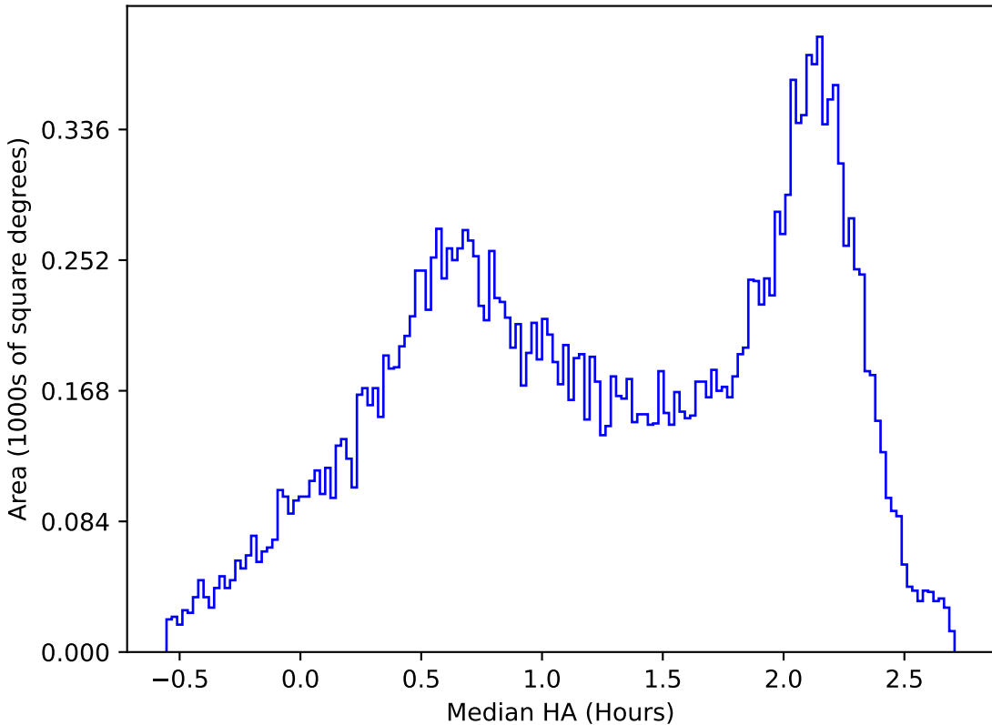
ddf_acor_sf10_ls40_lsr50_v3.4_10yrs All sky y band: Median HA
