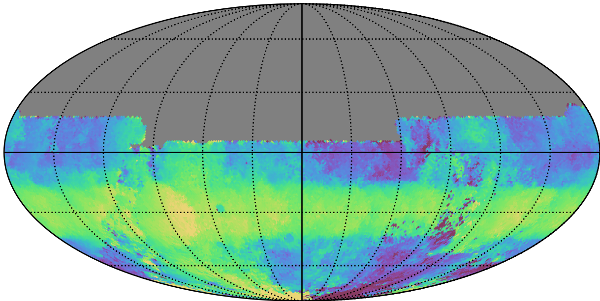
ddf_acor_sf10_lsf40_lsr50_v3.4_10yrs All sky u band: Median HA
